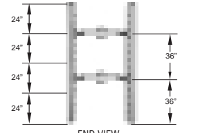
FULL LENGTH CORNER POST w/ADJUSTABLE STRUTS
