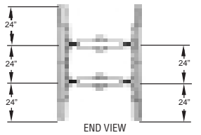
SECTIONAL CORNER POST w/ADJUSTABLE STRUTS.
