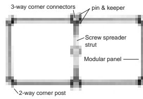
System using 3-way corner post
